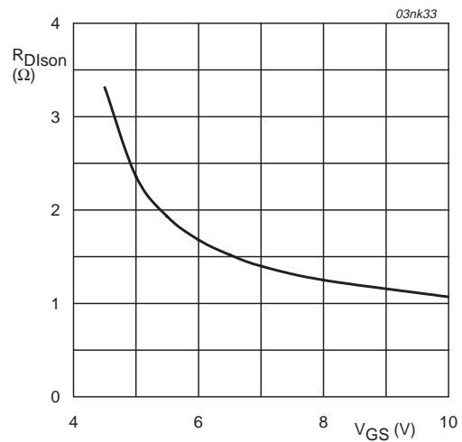
Fig 16. R_{Dlson} as function of gate-source voltage; typical values.
